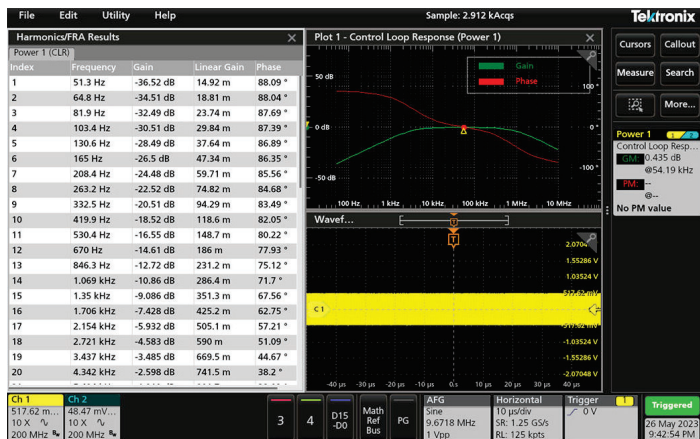
Frequency Response Analysis on the 2 Series MSO.
