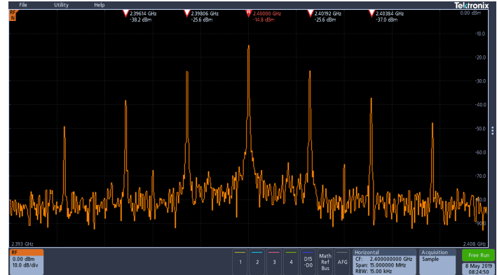
Automated peak markers identify critical information at a glance. As shown here, the five highest amplitude peaks that meet the threshold and excursion criteria are automatically marked along with each peak's frequency and amplitude.
