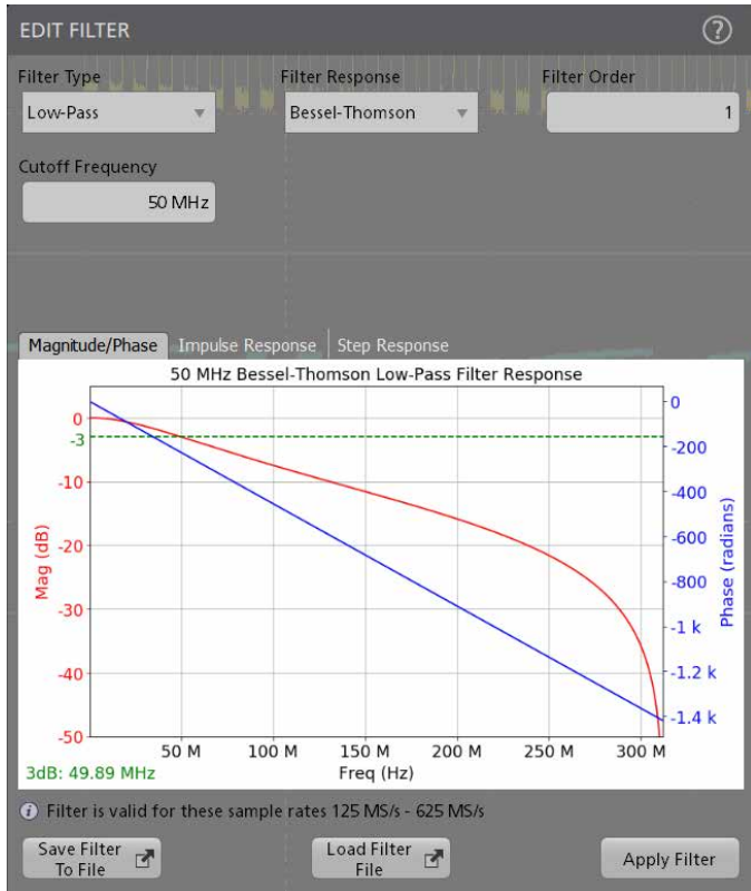
Filter creation dialog showing selection for Filter Type, Filter Response, Cutoff Frequency, Filter Order, and a graphical representation of Magnitude/Phase, Impulse Response, and Step Response
